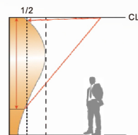
Light distribution of SILK Series wall washer.
