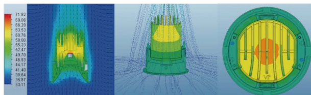
* ALPS Heat Release Simulation
